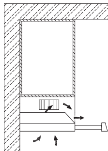
Recirculation mode (Double motors)
